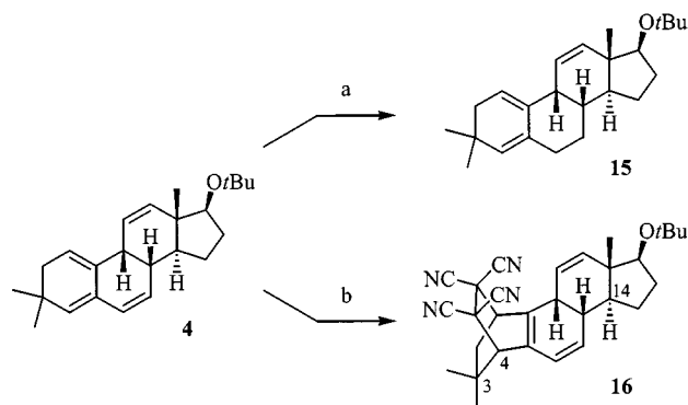
Scheme 6. Derivatization of steroid 4 by hydrogenation and Diels-Alder reaction: a) (\text{PPh}_3)_3\text{RhCl} , 3 bar \text{H}_2 , EtOAc, MeOH, 12 h, 84%; b) TCNE, toluene, reflux, 2 days, 74%
