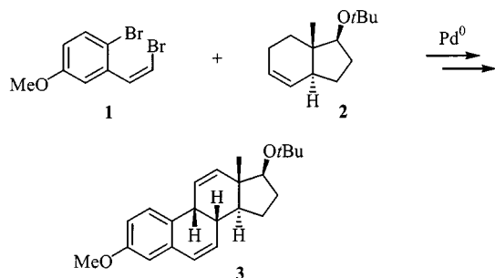
Scheme 1. Convergent synthesis of the estradiol derivative 3
