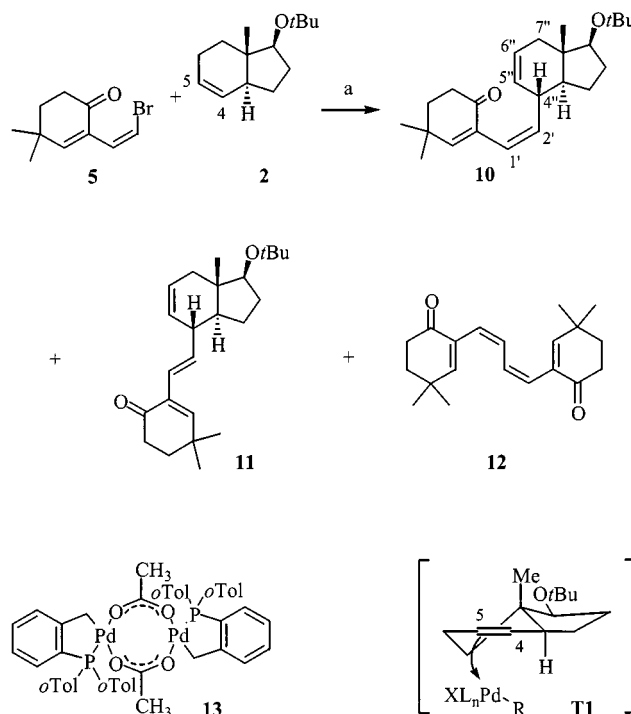
Scheme 4. Intermolecular Heck reaction of 5 and 2 : a) 1.0 mol-% 13 , n Bu 4 NOAc, DMF/CH 3 CN/H 2 O, 115 °C, 7 h, 56% ( Z )- 10 , 10% dimer 12 , traces ( E )- 11
