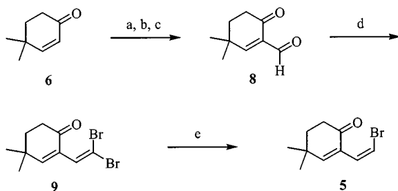
Scheme 3. Synthesis of 5 : a) H 2 , Pd/C, pentane, 24 h, 99%; b) NaH, HCO 2 Et, CyH, reflux, 4 h; CH 3 CO 2 H, 94%; c) DDQ, dioxane, room temp., 5 min., 76%; d) CBr 4 , PPh 3 , CH 2 Cl 2 , 0 °C → room temp., 2.5 h, 79%; e) n Bu 3 SnH, Pd(PPh 3 ) 4 , toluene, room temp., 2 h, 71%
