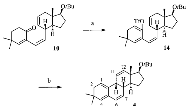
Scheme 5. Conversion of enone 10 to enol triflate 14 and subsequent Pd-catalyzed cyclization to estrane 4 : a) KHMDS, \text{TF}_2\text{NPh} , THF, -78^\circ\text{C} , 30 min., 94%; b) \text{Pd}(\text{dba})_2 , dppb, KOAc, DMAC, 75^\circ\text{C} , 18 h, 85%
