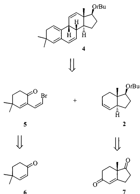
Scheme 2. Retrosynthetic analysis of the estrane 4
